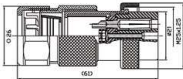
PLT-25-WGPF3-R 3=轉接3/8"尼龍管 Connected with 3/8"nylon tube
