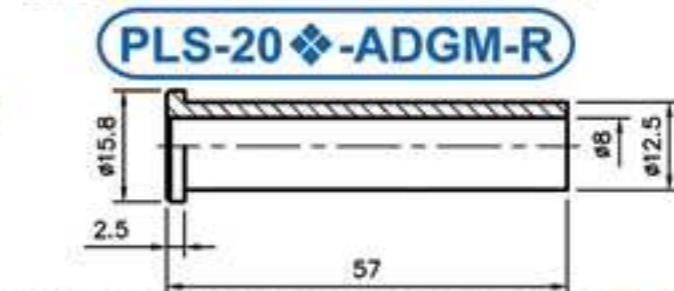
RUBBER TUBE FOR PLS-20-PF
