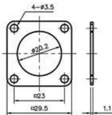
RUBBER GASKET FOR PLS-20-RM
