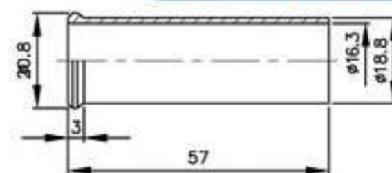
RUBBER TUBE : ACCESSORY FOR PLS-35-P
