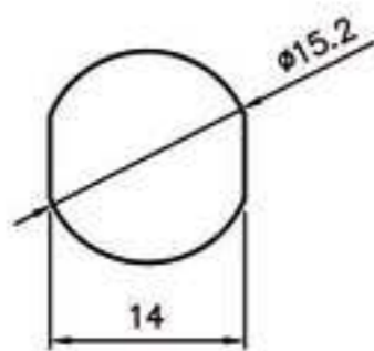
MOUNTING HOLES
