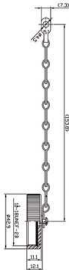
PLS-35-GPF6-R 6=轉接3/4"軟管 Connected with 3/4" conduit
