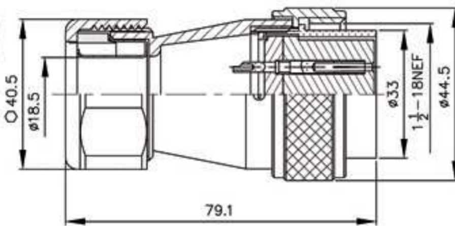
PLS-35-GPF6-R 6=轉接3/4"軟管 Connected with 3/4" conduit
