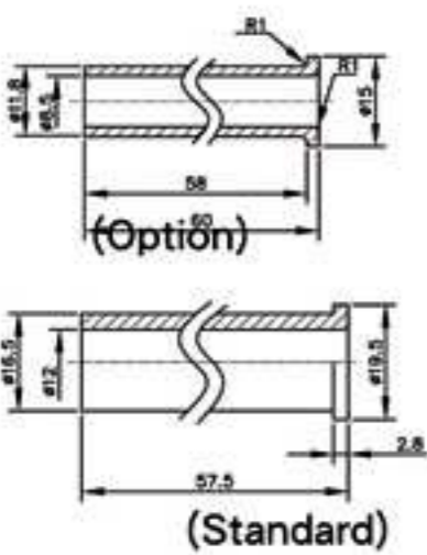
RUBBER TUBE FOR PLS-28-PM
