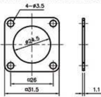
RUBBER GASKET FOR PLS-24-RF
