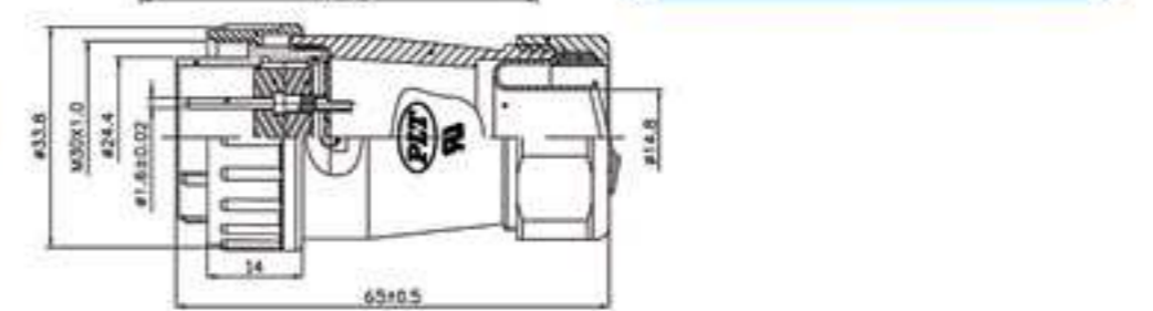
PLS-28-GPM4 X-R 4=轉接1/2"軟管 Connected with 1/2"conduit
