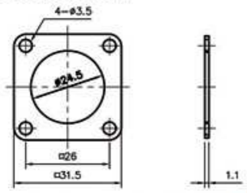
RUBBER GASKET FOR PLS-24-RM
